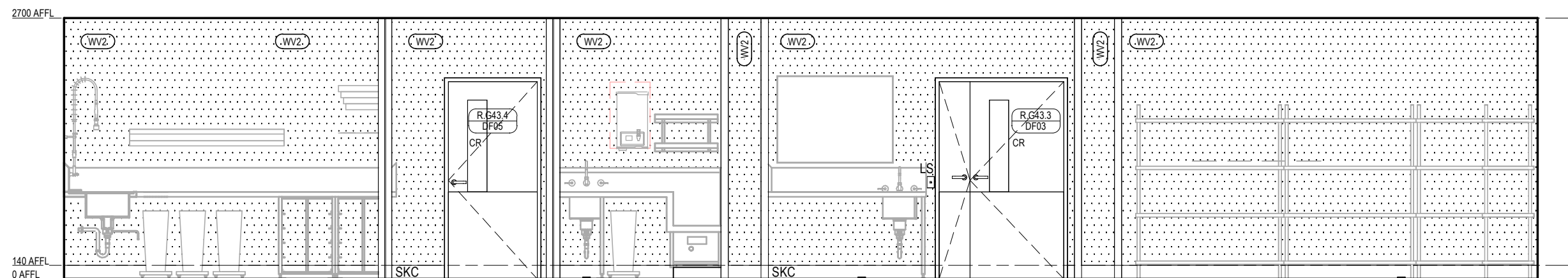
MAIN KITCHEN ELEVATION 3 Scale 1: 50
