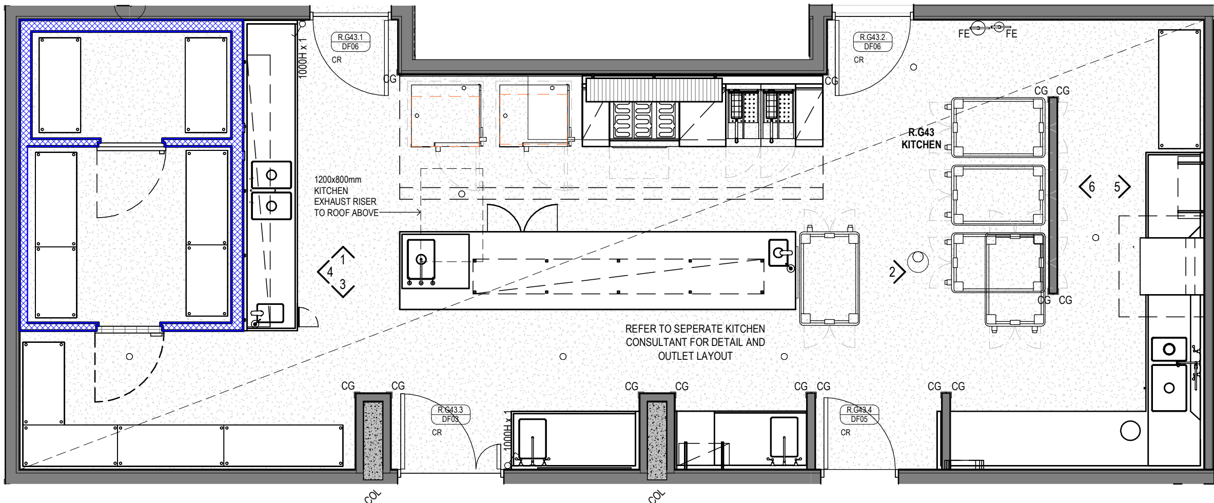
1 MAIN KITCHEN Scale 1: 50
