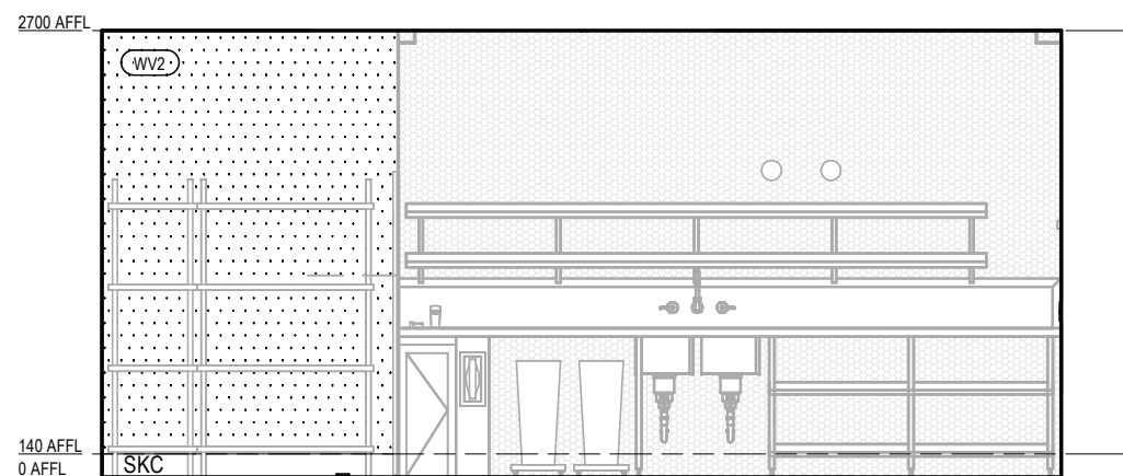
MAIN KITCHEN ELEVATION 4 Scale 1: 50
