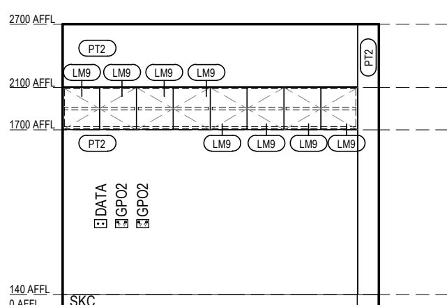
CHEF'S OFFICE ELEVATION 3 Scale 1: 50
