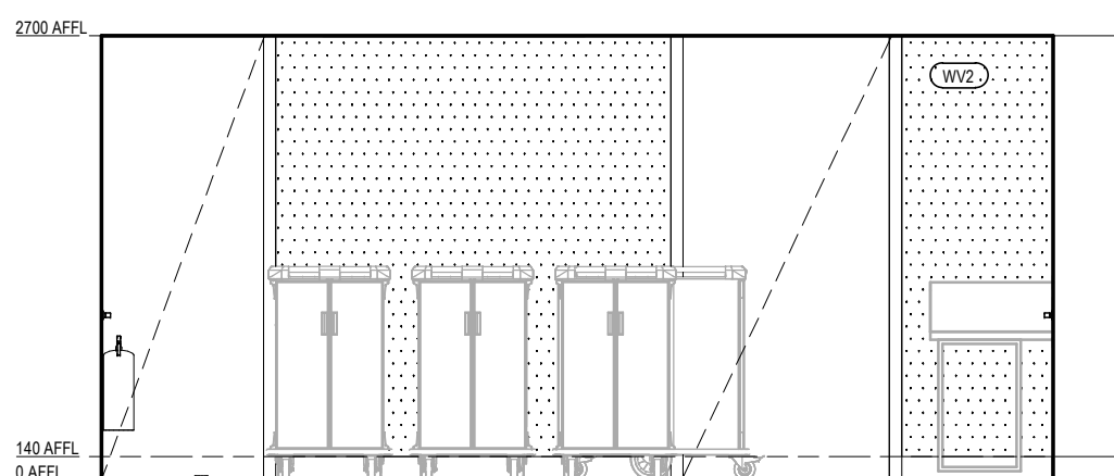
MAIN KITCHEN ELEVATION 2 Scale 1: 50
