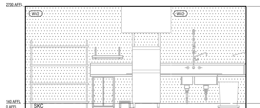
MAIN KITCHEN ELEVATION 5 Scale 1: 50
