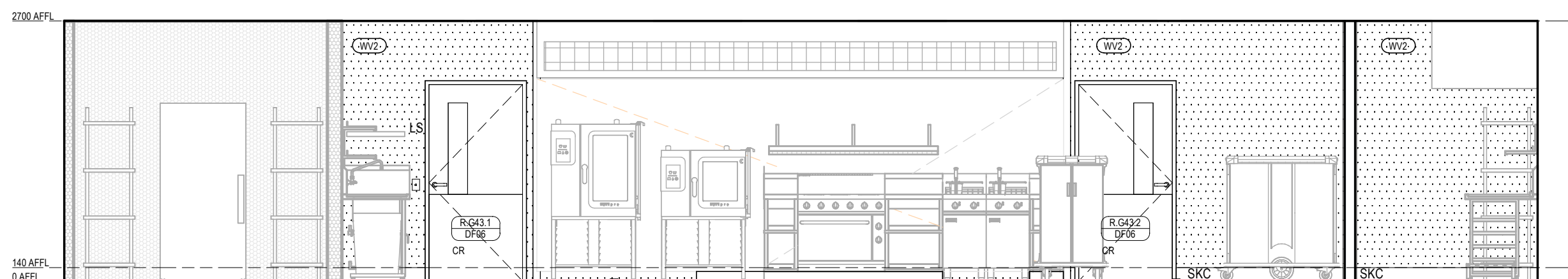
MAIN KITCHEN ELEVATION 1 Scale 1: 50
